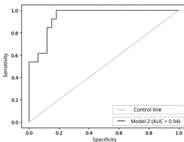
Fig. 6. ROC curve for model 2 with included NT-proBNP and sST2
